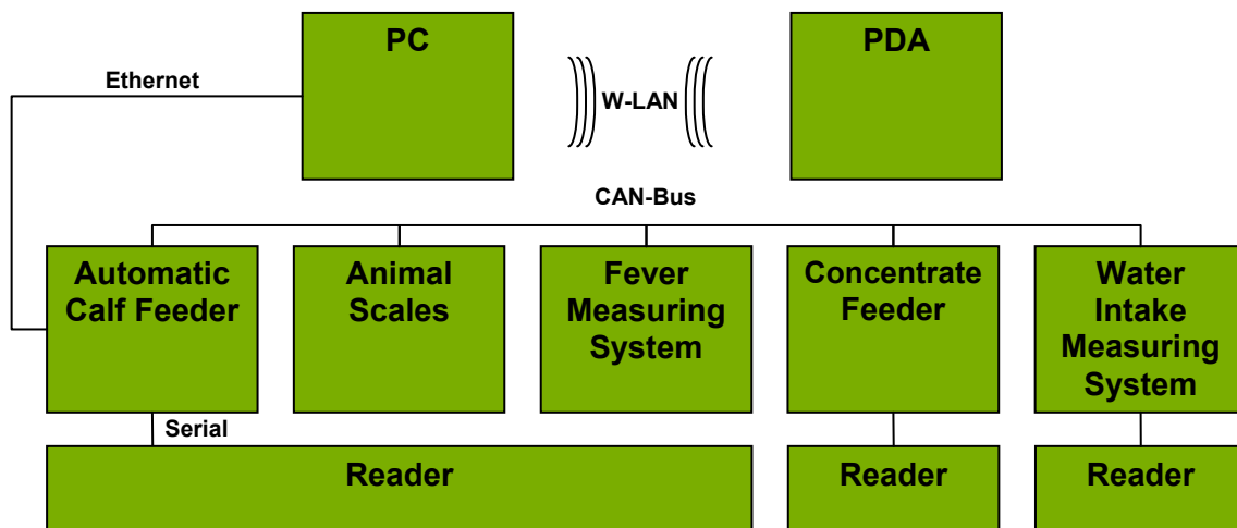
Figure 1. Components of a calf feeding system.
